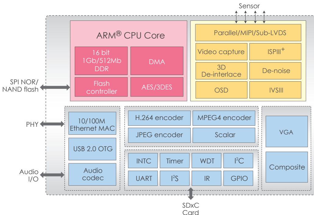
GM8136S/GM8135S SoC Block Diagram
